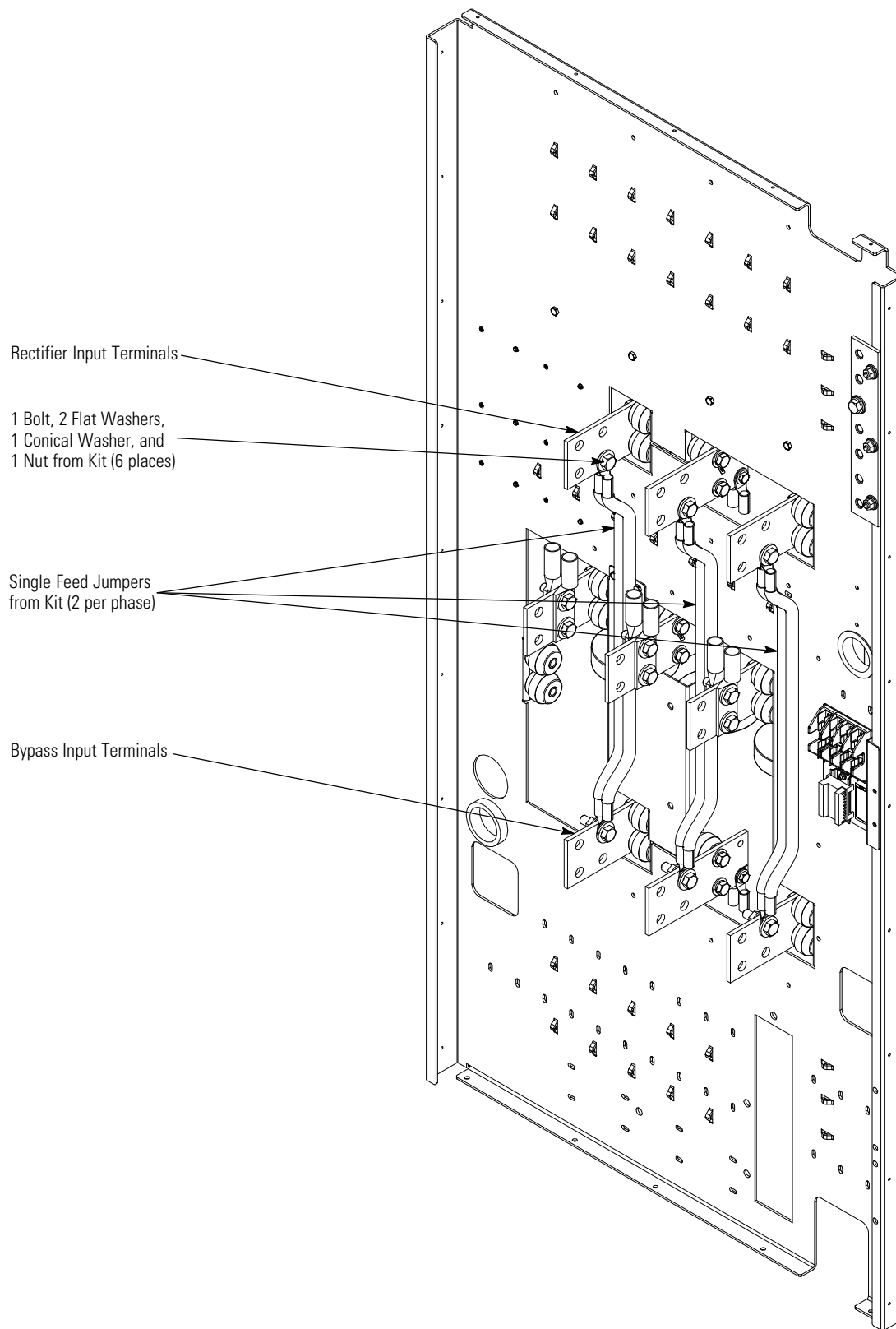
Figure 1. Eaton 9395 UPS (225–300 kVA) Single Feed Kit
